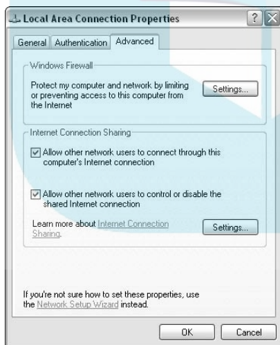
Figure 9-11: Enable Internet connection sharing in Windows XP.
